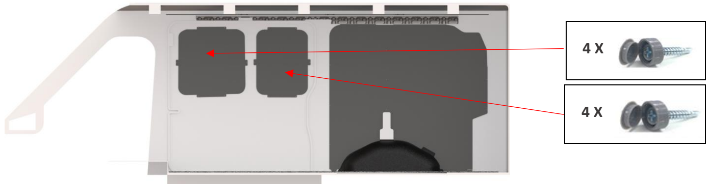
Figure 18 "Passenger Side Barn Door Liner Installed"
