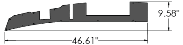
PASSENGER SIDE FRONT WALL LINER (P1A)
