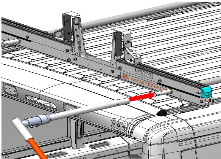
Step 17. Install and tighten the handle assembly Using a 1/2" wrench and 1/2" impact wrench, 5/16" x 2" bolts with the 5/16" washers and 5/16" lock nuts 02P168.
