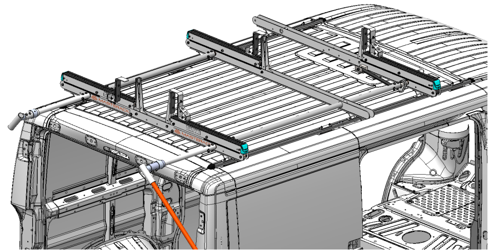
Step 18. Assembly after installation
