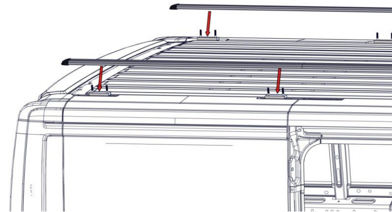
Step 7. Place the rail on top of the base brackets.
