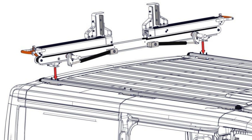
Step 12. Install rear crossbow over base brackets and tighten 4 5/16" nuts (02P168)
