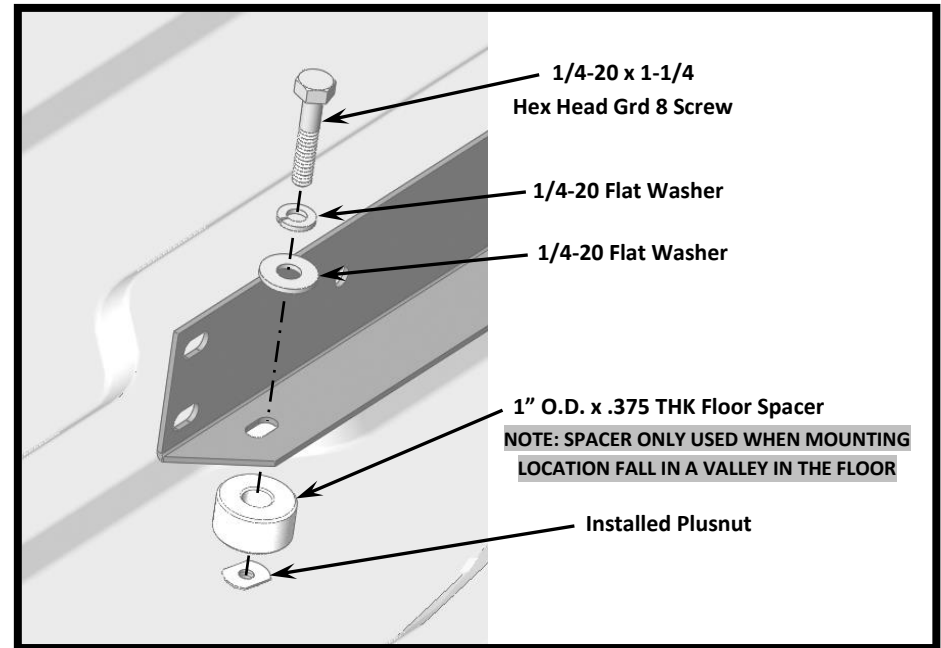
MOUNTING WITH PLUSNUT (LIMITED SPACE UNDER VEHICLE) (SEE PAGE 12 FOR PLUSNUT INSTALLATION)
